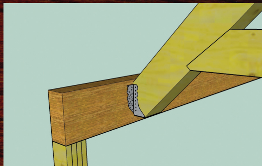
Hang trusses from beams using standard Simpson Strong-Tie® beam hangers.
