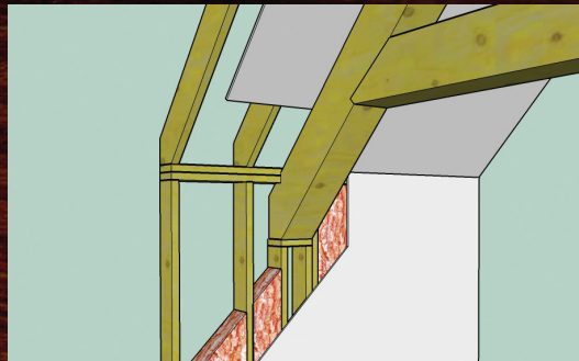
Simple in wall support system, can also be designed to sit on the top of the wall plate.
